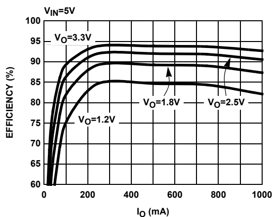
FIGURE 1. EFFICIENCY
