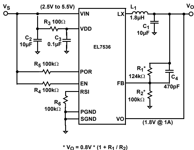
EL7536 TOP VIEW
