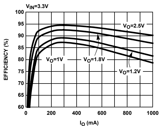
FIGURE 2. EFFICIENCY
