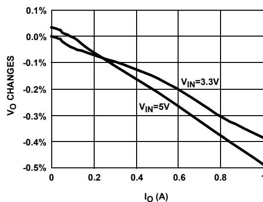
FIGURE 4. LOAD REGULATIONS
