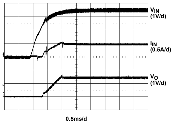
FIGURE 7. START-UP 1
