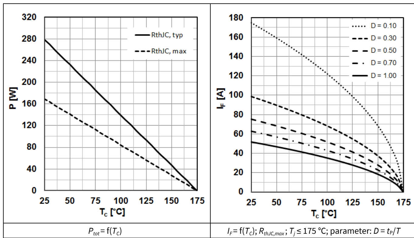
Figure 1 Power dissipation
