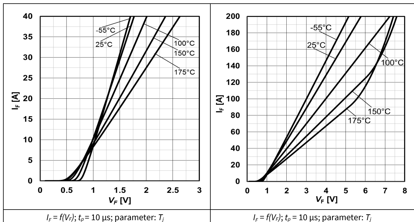
Figure 3 Typ. forward characteristics
