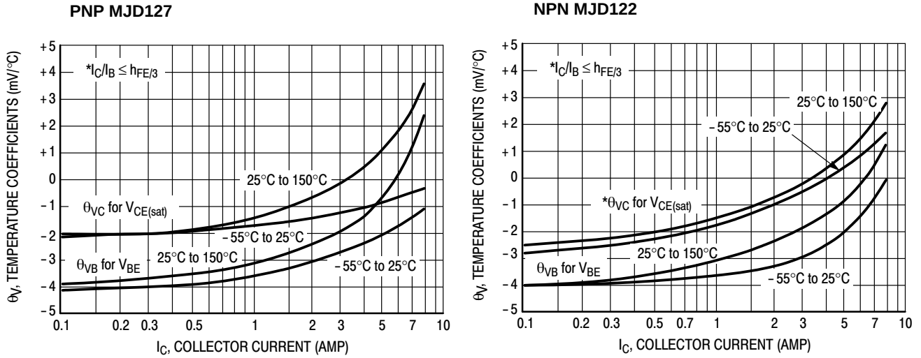
Figure 5. Temperature Coefficients
