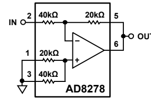
Figure 55. Inverting Amplifier, Gain = -1/2
