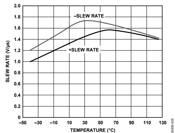
Figure 30. Slew Rate vs. Temperature, V_{IN} = 20\text{ V p-p} , 1 kHz
