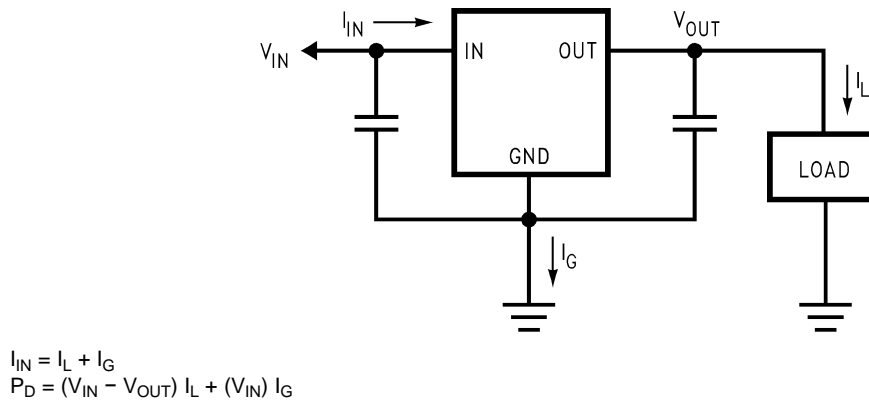
Figure 25. Power Dissipation Diagram
