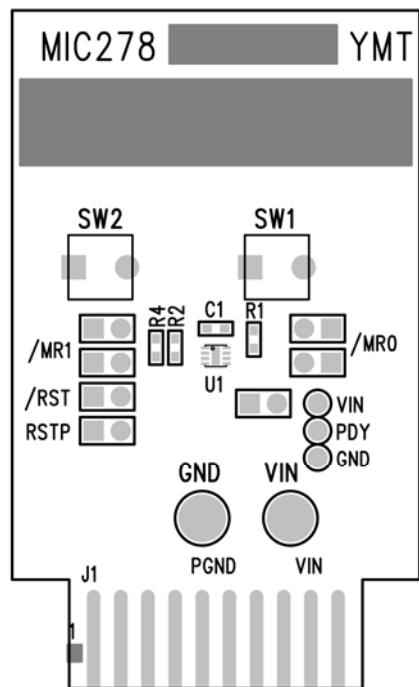
Top Silkscreen
