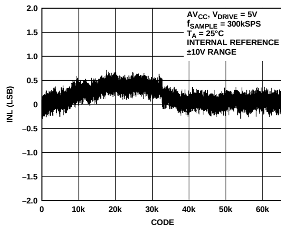
Figure 11. Typical INL, \pm 10\text{ V} Range
