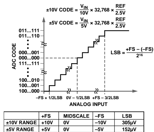
Figure 33. Transfer Characteristics
