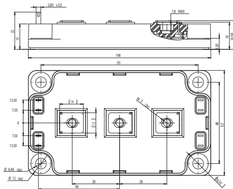
SP6–Three Outputs
