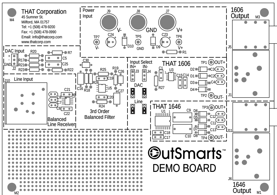
Assembly Drawing
