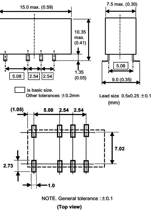
High solder joint reliability/ Non-latch type, Single coil latch type
