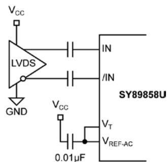
Figure 3f. LVDS Interface (AC-Coupled)
