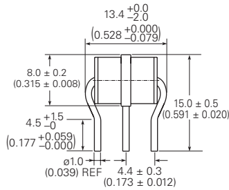
Axial Leaded (GTCA38-XXXM-R10)
