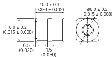
Surface-mount (GTCS38-XXXM-R10)
