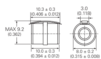
No Leads with-FT (GTCN38-XXXM-R10-FT)†
