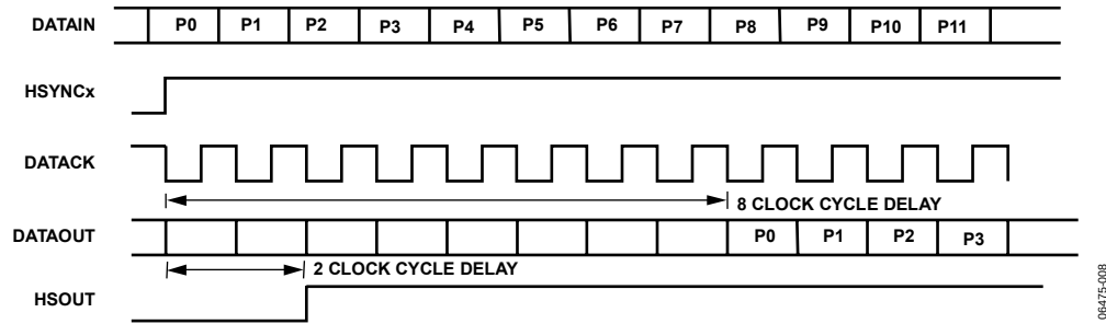
Figure 14. 4:4:4 Timing Mode
