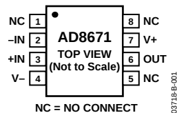
Figure 1. 8-Lead SOIC-N (R-8) and 8-Lead MSOP (RM-8)
