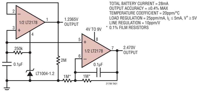
Self-Buffered, Dual Output, Micropower Reference
