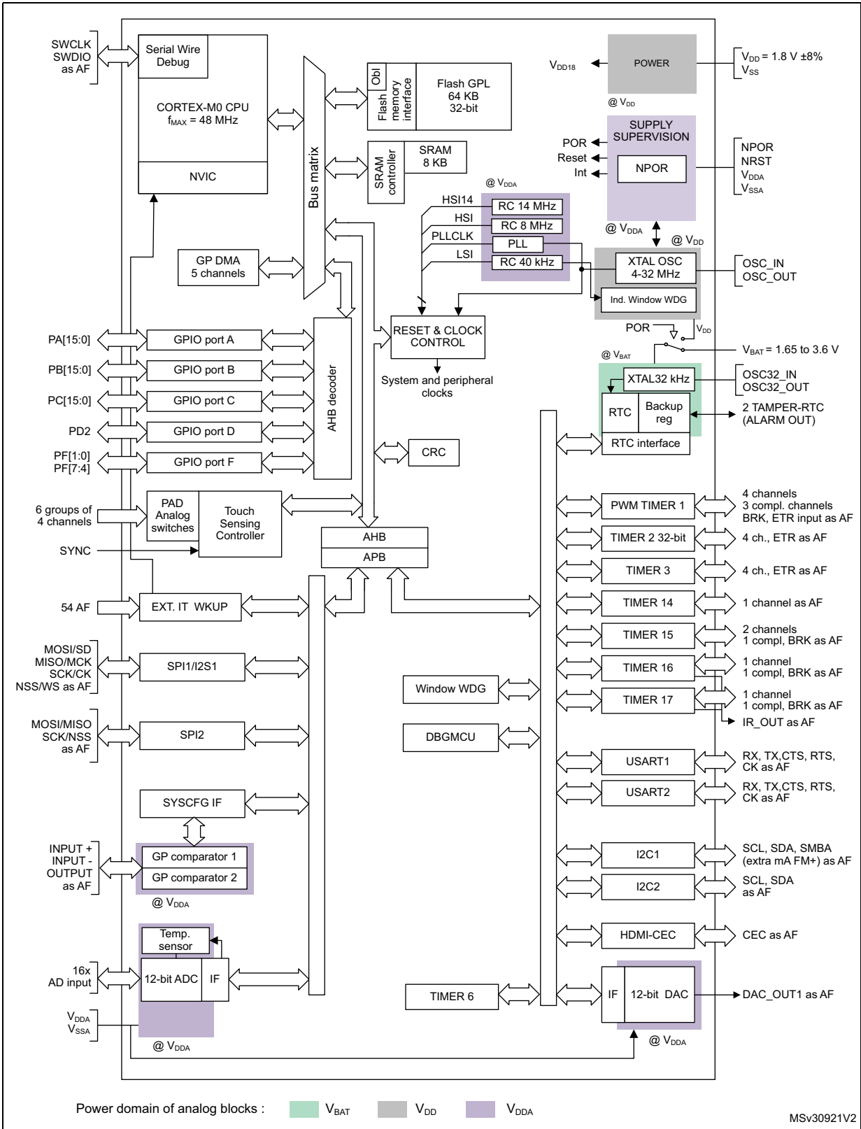
Figure 1. Block diagram
