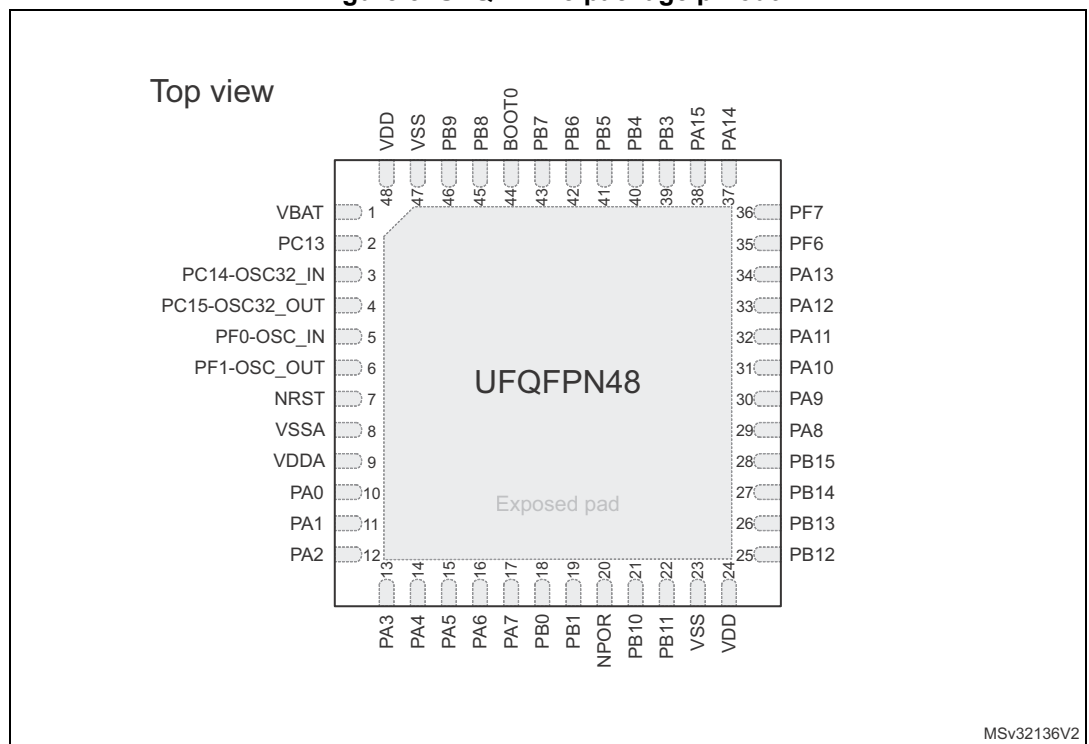
Figure 5. UFQFPN48 package pinout
