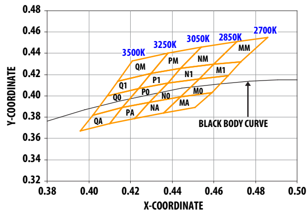
Figure 3 Color Bin Structure for Warm White
