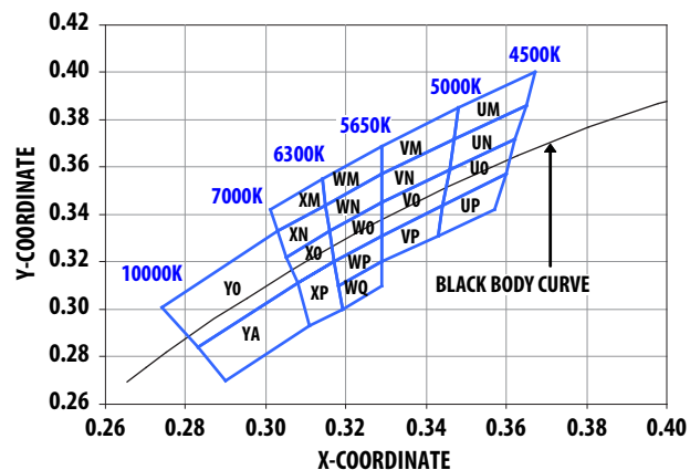
Figure 2 Color Bin Structure for Cool White
