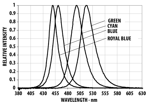
Figure 16 Relative Intensity vs. Wavelength for Blue, Royal Blue, Cyan, and Green
