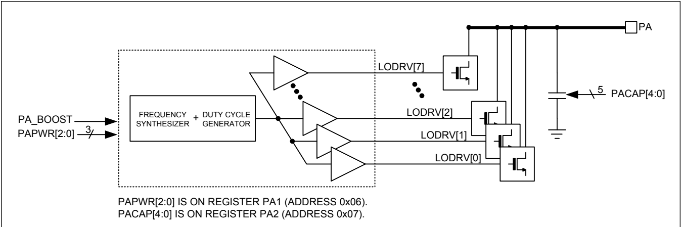
Figure 2. Power Amplifier
