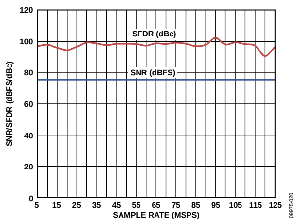
Figure 18. SNR/SFDR vs. Sample Rate with AIN = 9.7 MHz
