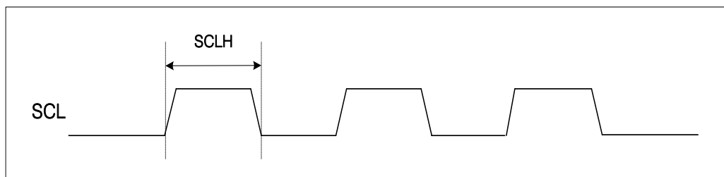
Figure 15.3.SCL HIGH Timing
