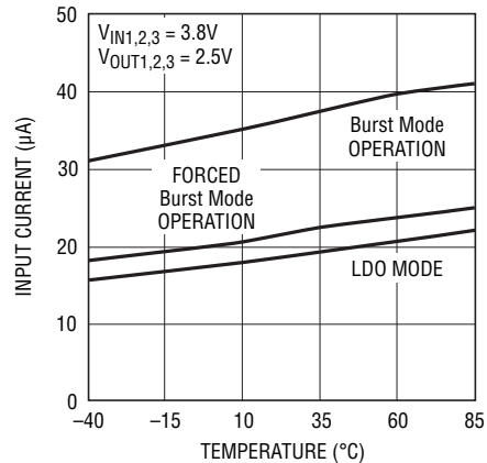
Switching Regulator Low Power Mode Quiescent Currents
