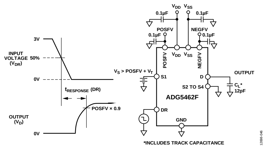
Figure 47. Drain Enable Time with Overvoltage, t_{RESPONSE (DR)}
