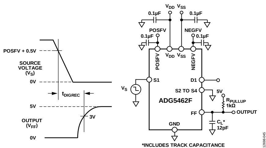
Figure 46. Interrupt Flag Recovery Time, t_{DIGREC} , with a 1 kΩ Pull-Up Resistor
