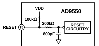
Figure 26. Power-On Reset
