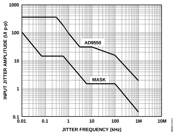
Figure 25. Jitter Tolerance
