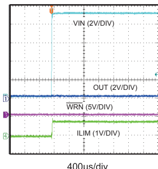
Zoom In View of Power-up Waveform when Output is Short-circuit
