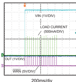
Power-up Waveform when Output is Short-circuit
