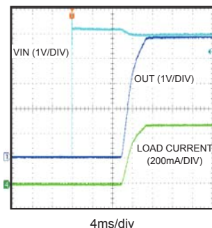
Input Power Up Waveform Output loaded with 10 \Omega resistor
