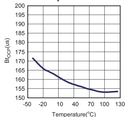
Overcurrent Protection Blanking Time vs. Temperature
