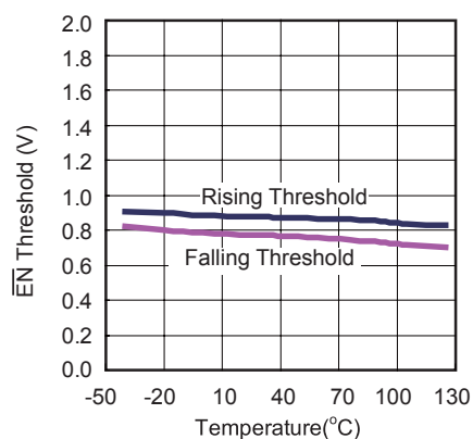
\overline{EN} Input Threshold vs. Temperature
