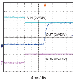
Input Steps From 6.5V to 5.5V Waveform
