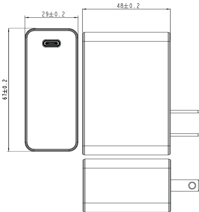
AQ36A-5CFA-H Dimension Diagram Unit: mm
