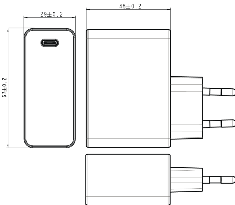
AQ36E-5CFA-H Dimension Diagram Unit: mm
