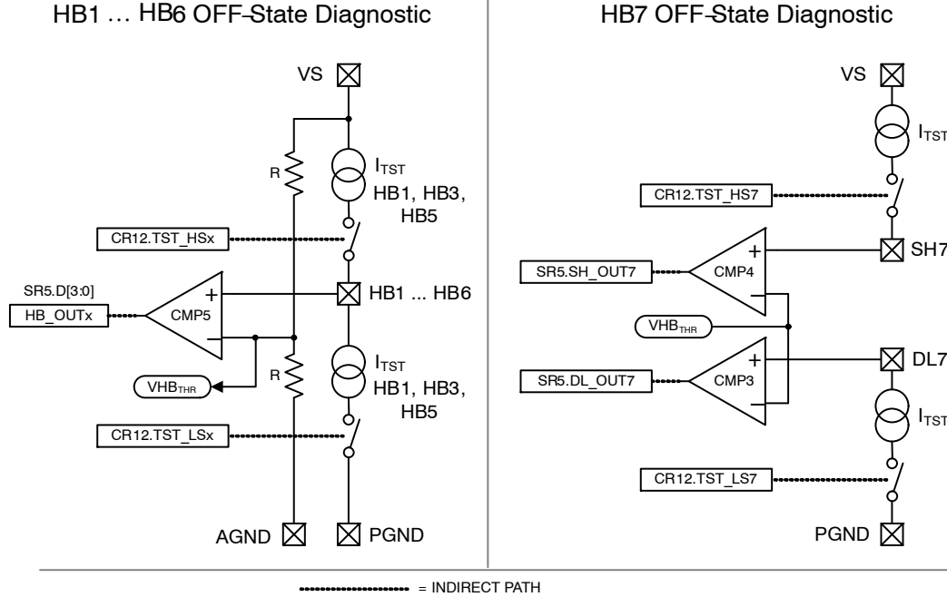
Figure 17. Half-bridge OFF-state Diagnostic
