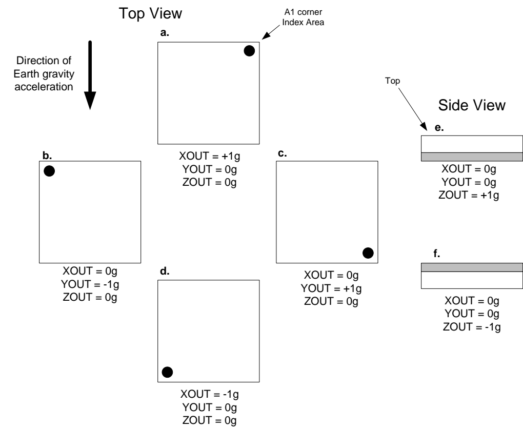
Figure 3. Package Orientation
