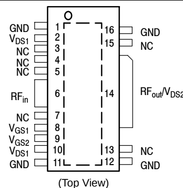
Figure 2. Pin Connections
