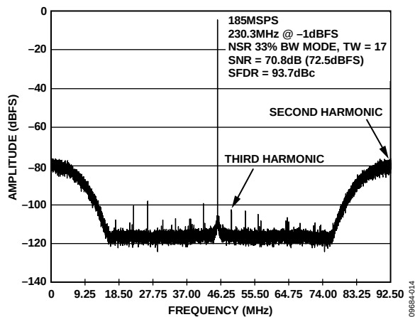
Figure 14. Single Tone FFT, f_{IN} = 230.3 MHz, NSR Enabled in 33% BW Mode, Tuning Word = 17
