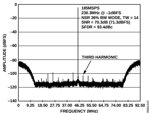
Figure 15. Single Tone FFT, f_{IN} = 230.3 MHz, NSR Enabled in 36% BW Mode, Tuning Word = 14
