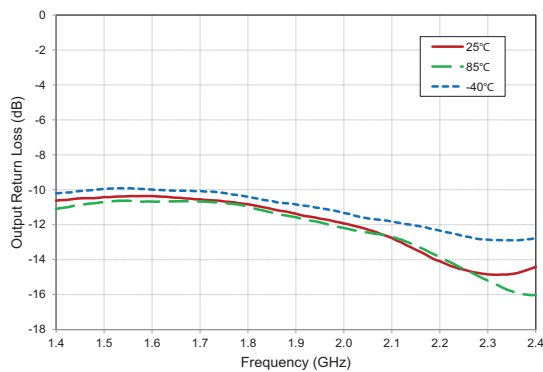
Output Return Loss Over Temperature
