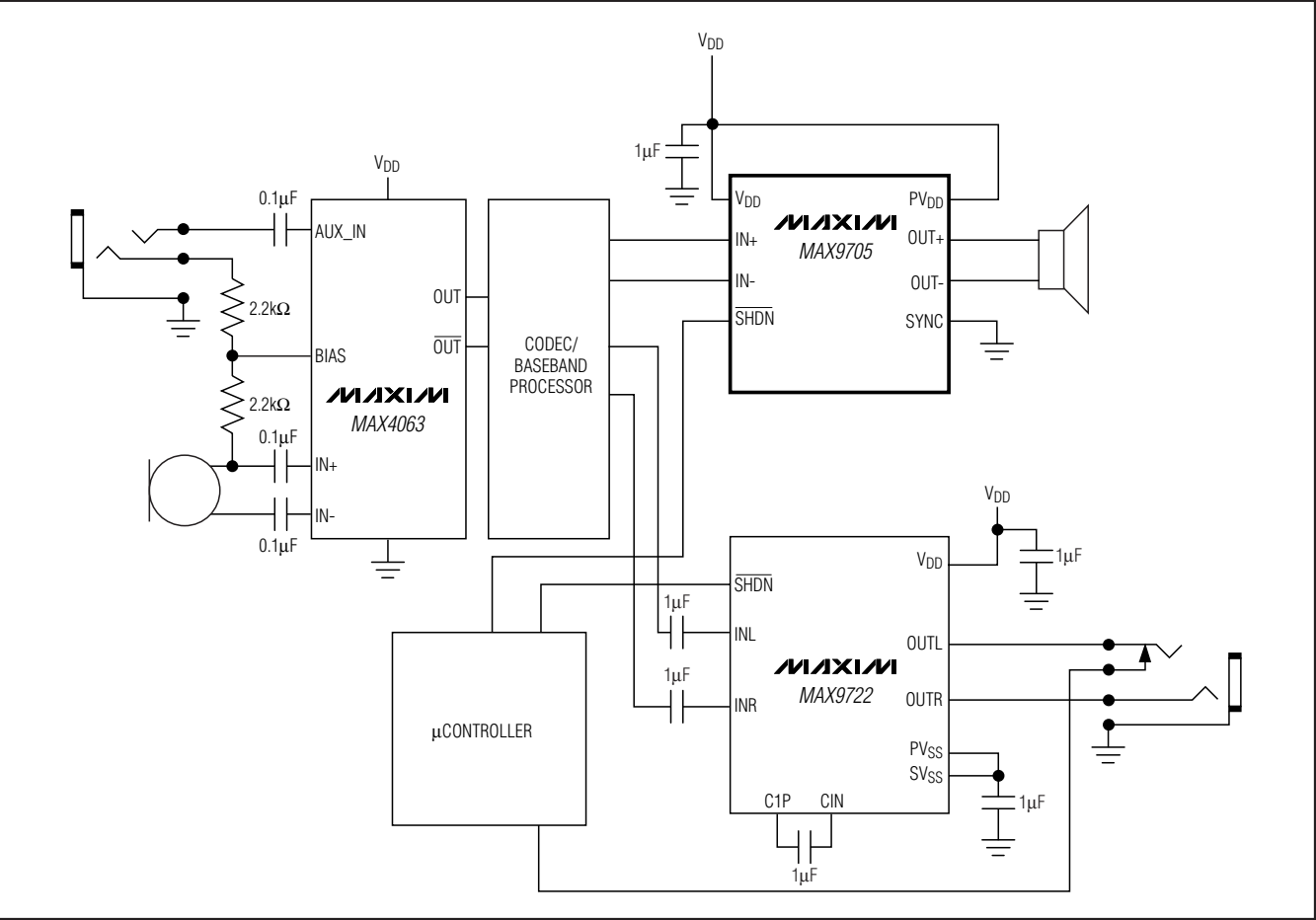
System Diagram
