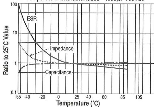
Temperature Characteristics - 4600 \mu F 100Vdc
