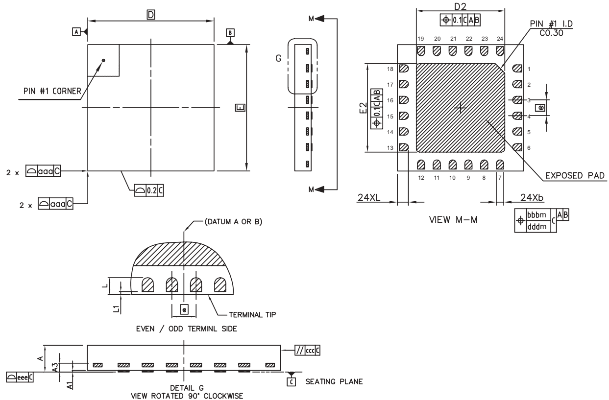
Figure 29. TQFN(4x4)-24 Package
