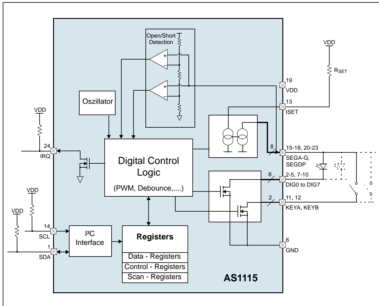
Figure 16. Block Diagram (QSOP-24 Package)
