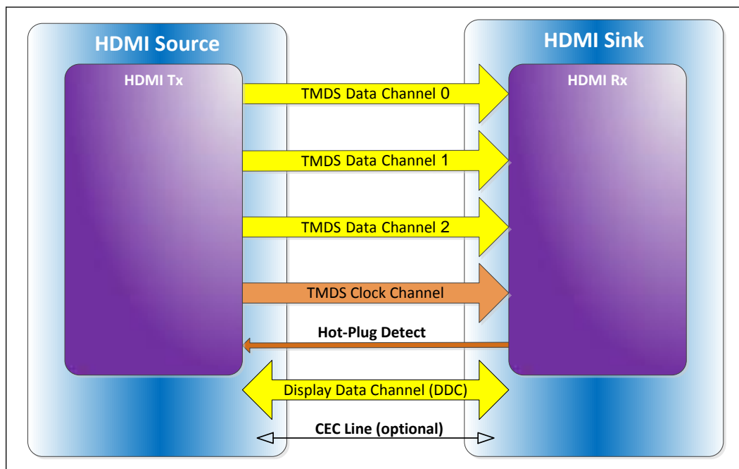
Figure 8. HDMI* Overview
