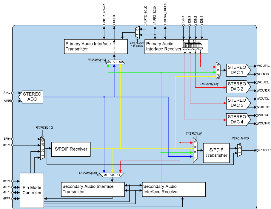
Figure 25 Digital Routing
