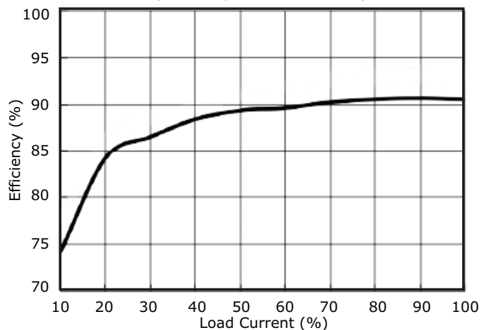
PDRA-120-12 Efficiency Curve (Efficiency vs. Load Current)
