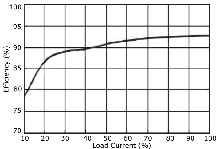
PDRA-120-24 Efficiency Curve (Efficiency vs. Load Current)
