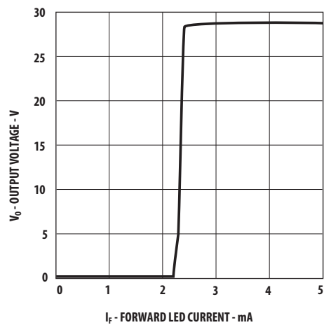
Figure 15 Transfer Characteristics
