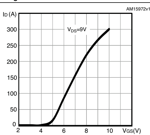
Figure 7. Transfer characteristics
