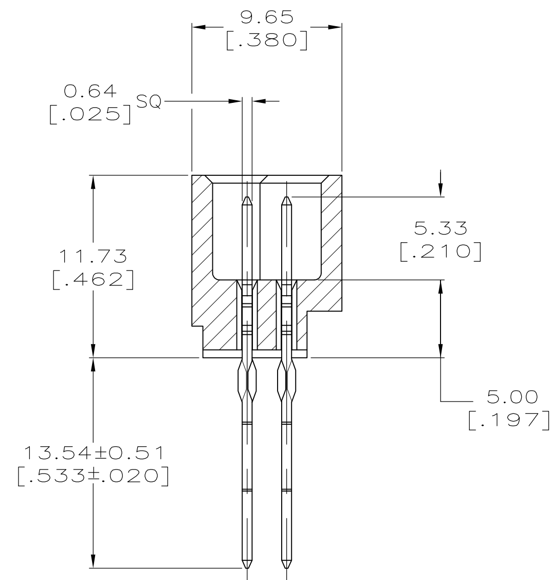
SECTION T-T
