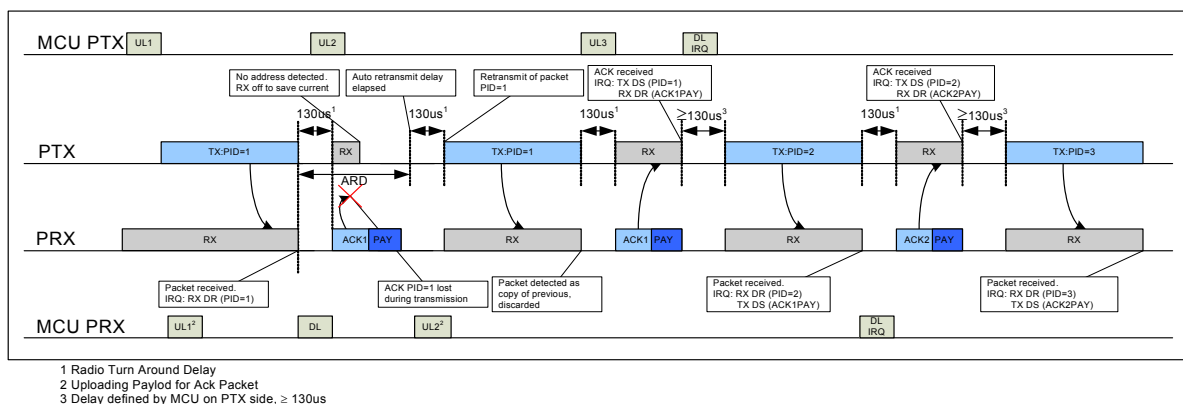
Figure 22. TX/RX cycles with ACK Payload and the according interrupts when the ACK packet fails
