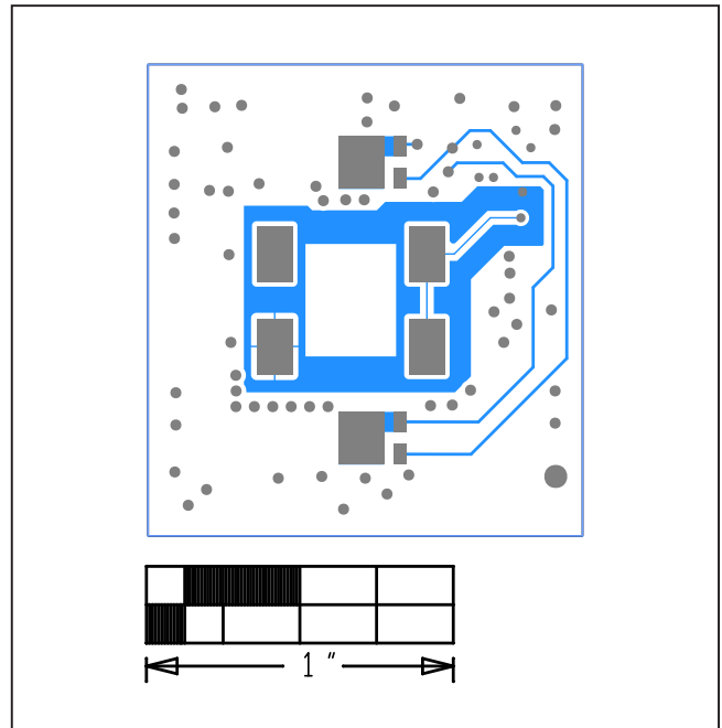
MAX86140OSBEK#—BOTTOM
