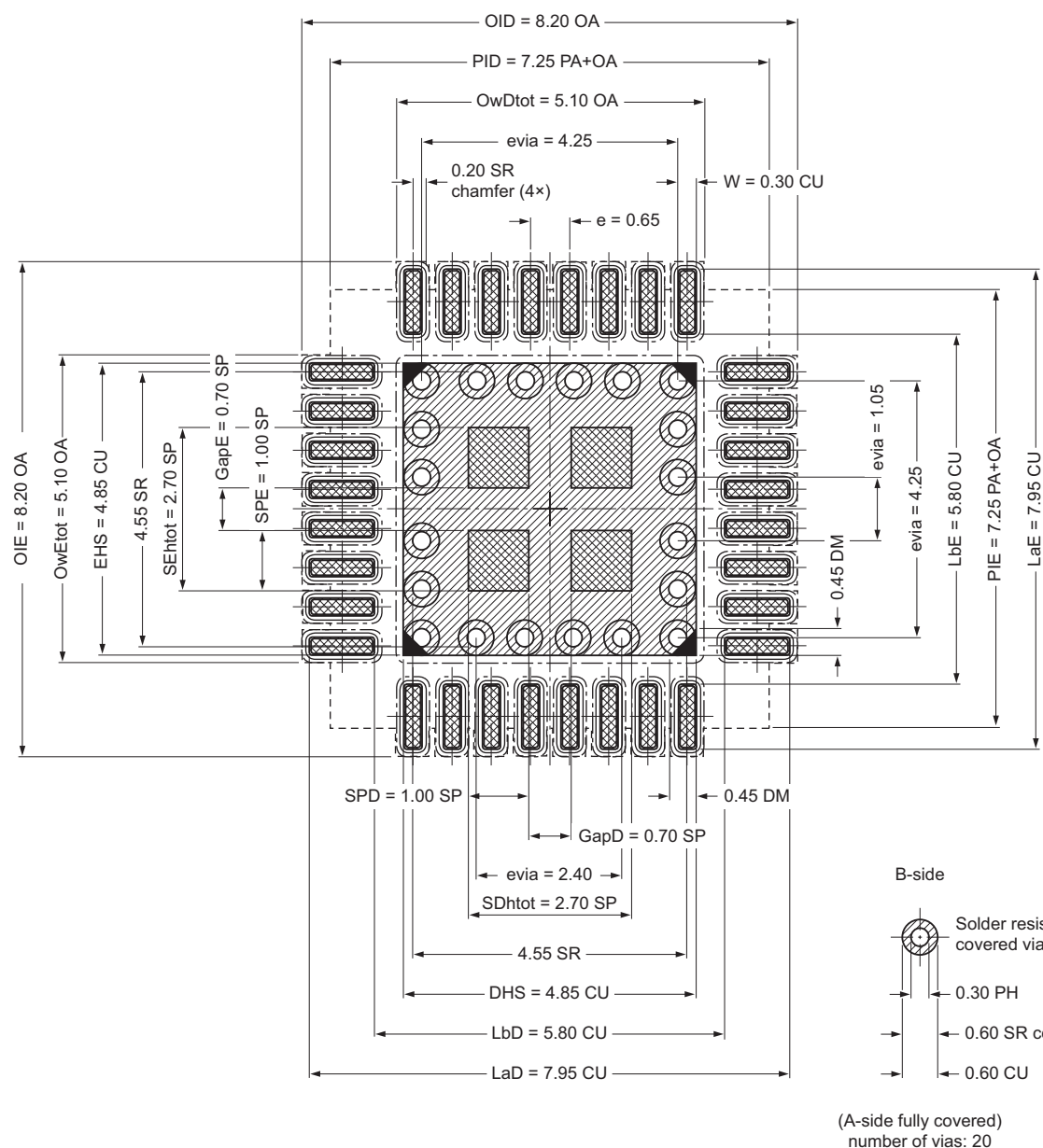
Footprint information for reflow soldering of HVQFN33 package
