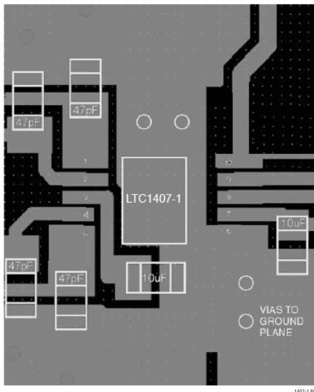
Figure 7. Recommended Layout
