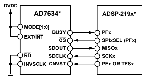
Figure 48. Interfacing the AD7634 to SPI Interface
