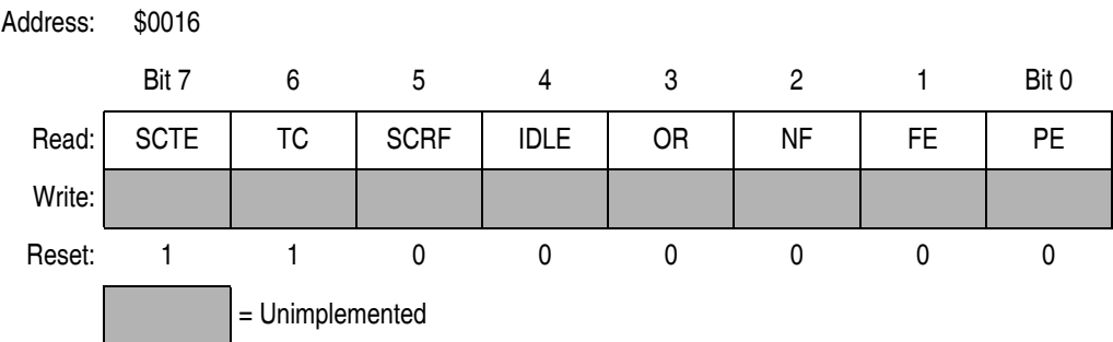
Figure 15-12. SCI Status Register 1 (SCS1)
