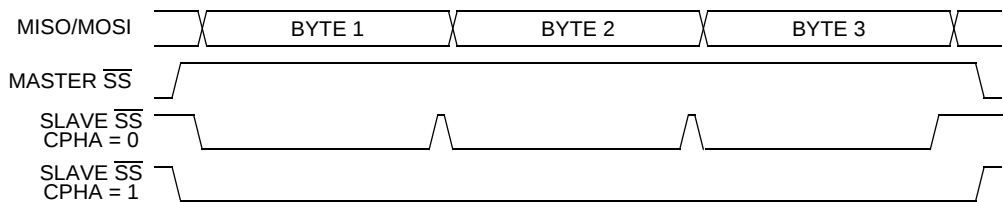
Figure 16-5. CPHA/SS Timing
