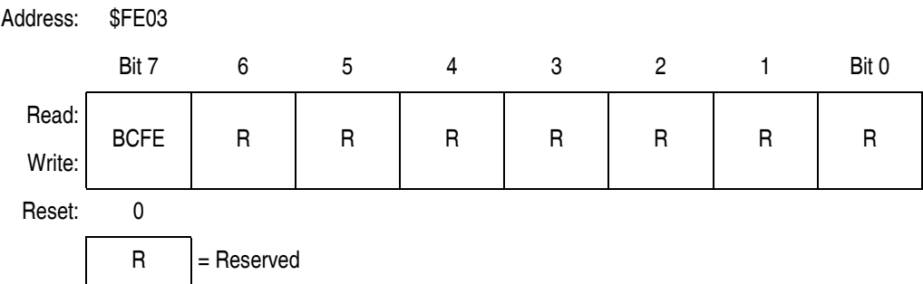
Figure 8-19. SIM Break Flag Control Register (SBFCR)
