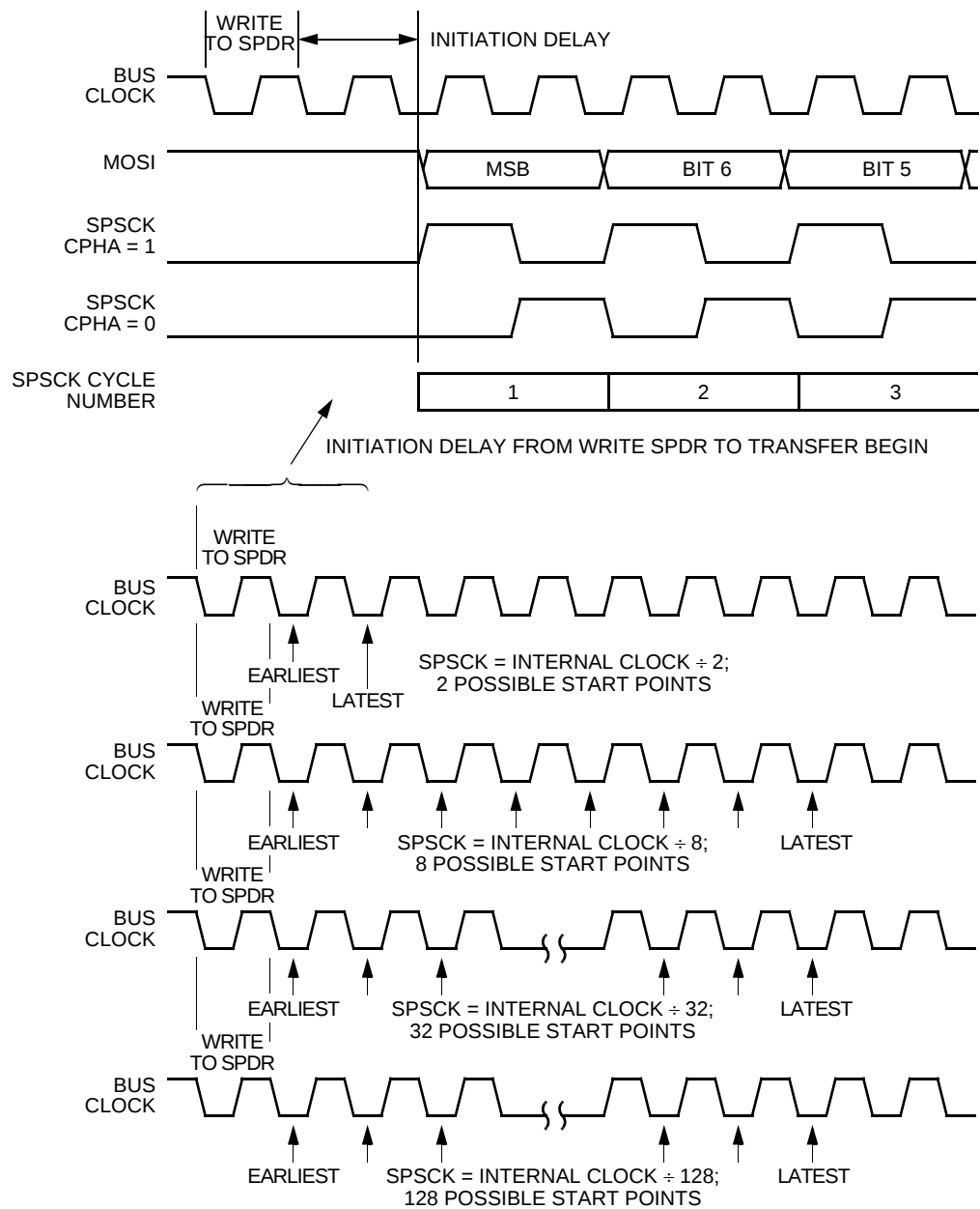
Figure 16-7. Transmission Start Delay (Master)
