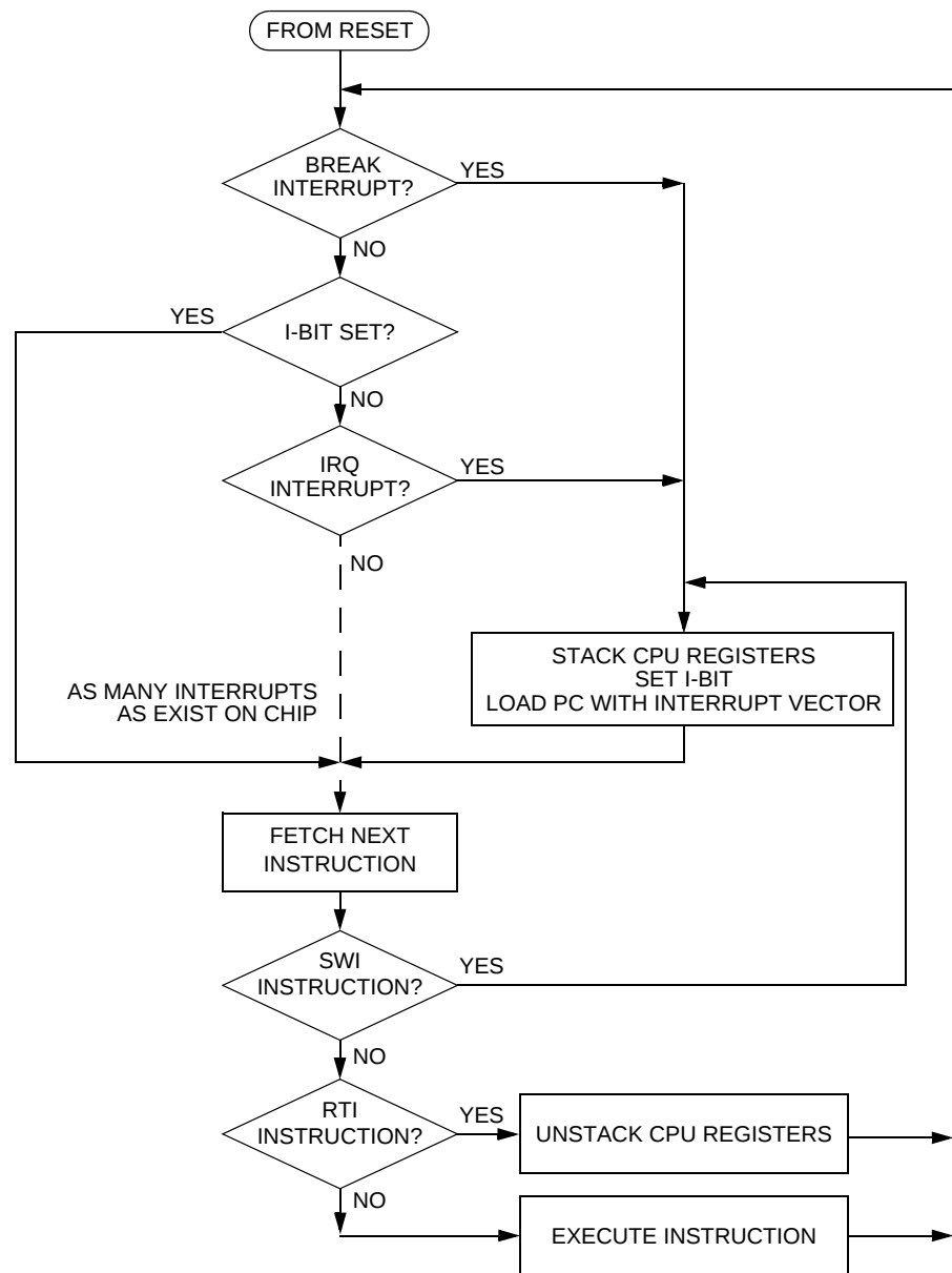
Figure 8-10. Interrupt Processing
