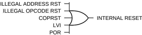
Figure 8-6. Sources of Internal Reset
