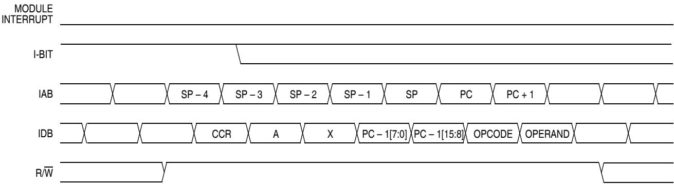
Figure 8-9. Interrupt Recovery Timing
