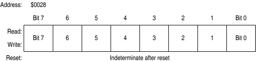
Figure 11-15. TIMA Channel 0 Register Low (TACH0L)
