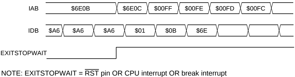
Figure 8-13. Wait Recovery from Interrupt or Break
