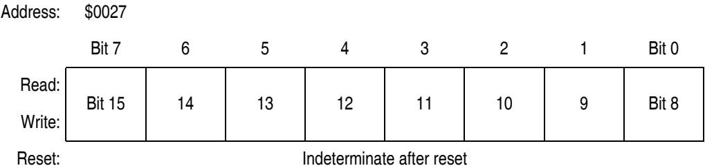
Figure 11-14. TIMA Channel 0 Register High (TACH0H)
