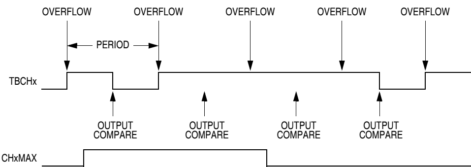
Figure 12-13. CHxMAX Latency
