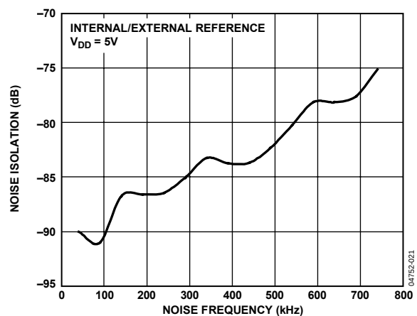
Figure 4. Channel-to-Channel Isolation
