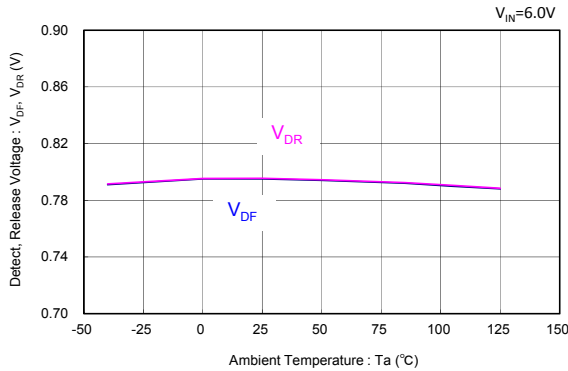
XC6134 ( V_{DF(T)}=0.8V )
