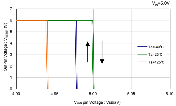
XC6134x50A ( V_{DF(T)}=5.0V )
