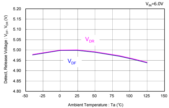
XC6134 ( V_{DF(T)}=5.0V )
