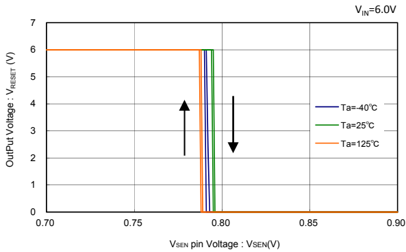
XC6134x08A ( V_{DF(T)}=0.8V )
