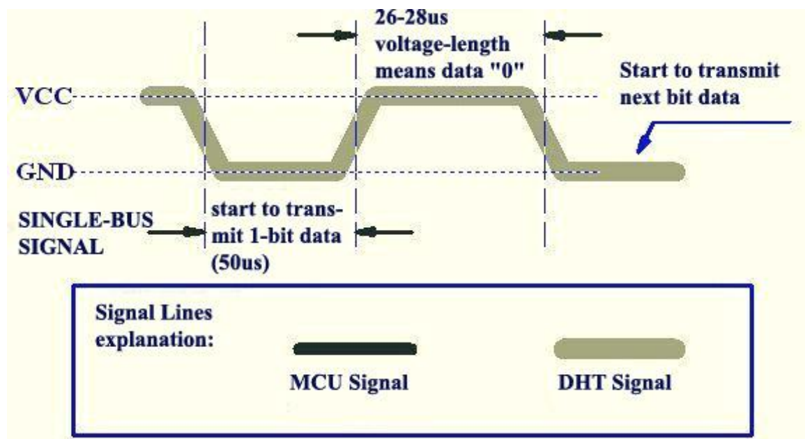
Figure 4 Data "0" Indication
